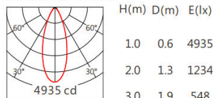
JR-5050 40° 3000K
