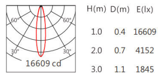
JR-5050 20° 4000K
