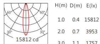
JR-5050 20° 3000K
